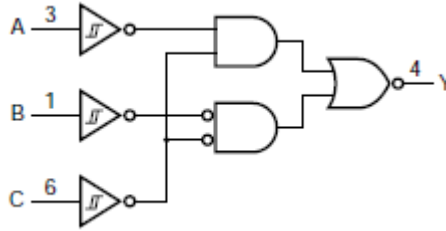
Figure 1. Logic symbol
