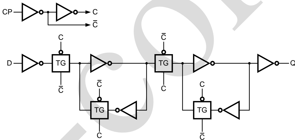
Figure 3. Logic diagram
