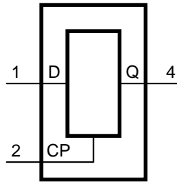
Figure 1. Logic symbol
