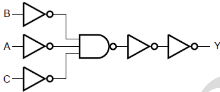
Figure 1. Logic symbol
