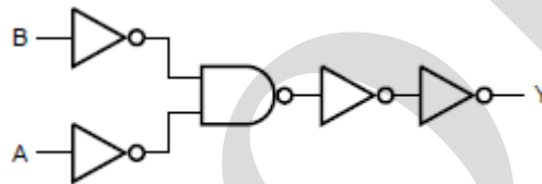
Figure 3. Logic diagram (one gate)
