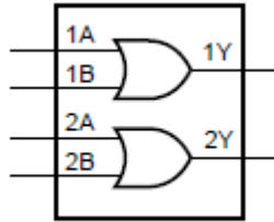
Figure 1. Logic symbol
