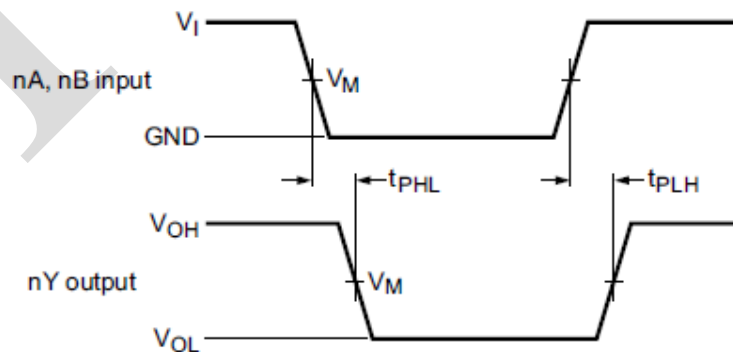
Figure 4. The input (nA, nB) to output (nY) propagation delays
