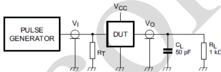
Figure 3. Test circuit for switching times
