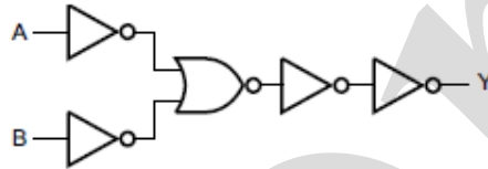
Figure 2. Logic diagram (one gate)
