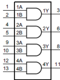
Figure 1. Logic symbol
