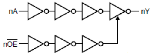
Figure 3. Logic diagram (one buffer)
