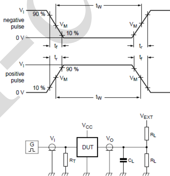
Figure 4. Load circuit for switching times
