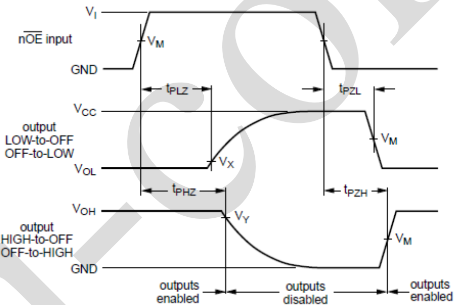
Figure 6. Enable and disable times
