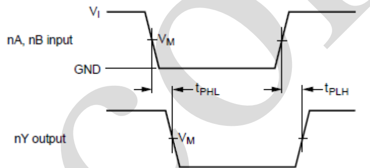
Figure 5. The input (nA, nB) to output (nY) propagation delays
