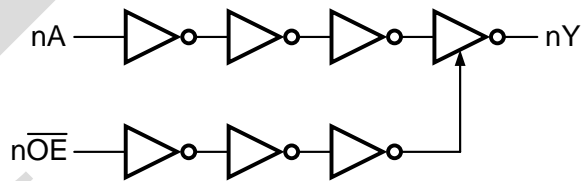
Figure 3. Logic diagram
