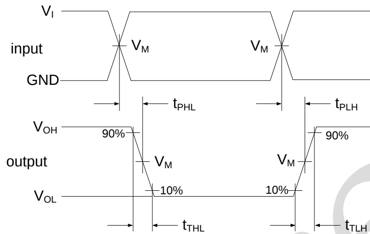
Figure 3. The data input (A or B) to output (Y) propagation delays
