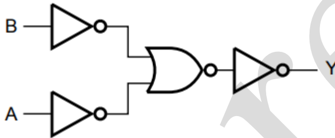
Figure 2. Logic diagram
