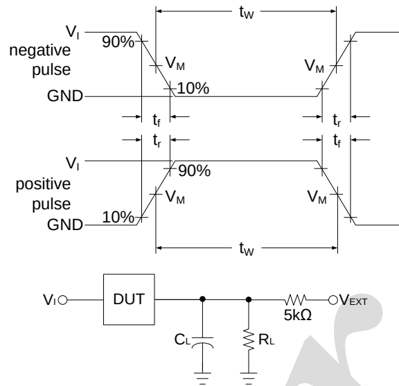
Figure 3. Test circuit for measuring switching times
