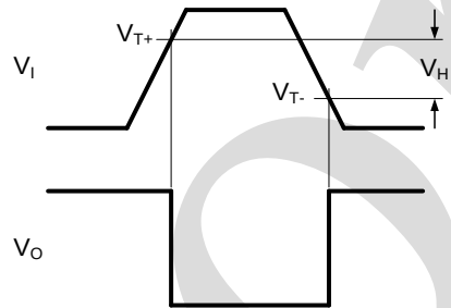
Figure 7. Definition of V_{T+} , V_{T-} and V_H
