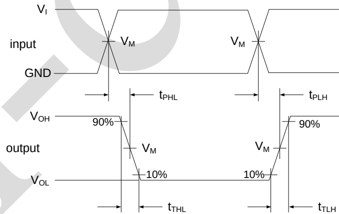
Figure 5. The input A to output Y propagation delays
