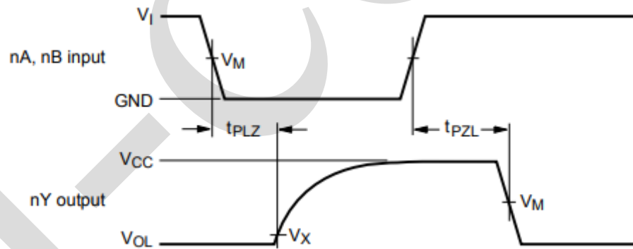
Figure 4. The input nA, nB to output nY propagation delays
