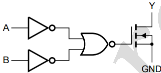
Figure 2. Logic diagram (one Schmitt trigger)
