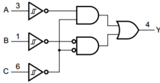
Figure 1. Logic symbol
