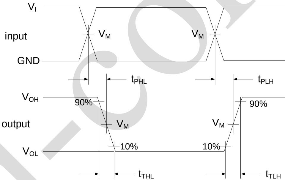
Figure 3. The data input (nA or nB or nC) to output (nY) propagation delays
