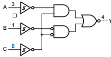
Figure 1. Logic symbol
