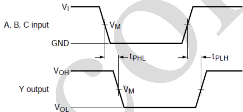
Figure 4. The data input (A, B or C) to output (Y) propagation delays
