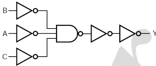
Figure 2. Logic diagram
