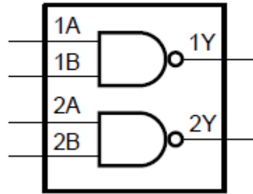
Figure 1. Logic symbol
