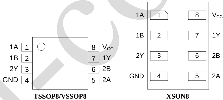
Figure 3. Pin configurations
