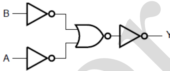
Figure 2. Logic diagram
