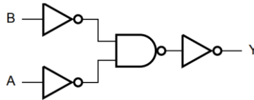
Figure 2. Logic diagram
