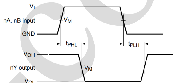
Figure 4. The data input (nA, nB) to output (nY) propagation delays
