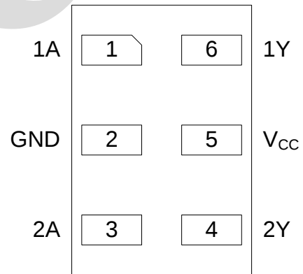
XSON6
