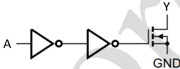
Figure 2. Logic diagram (one gate)
