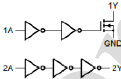
Figure 2. Logic diagram
