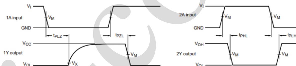
Figure 4. The data input 1A to output 1Y and input 2A to output 2Y propagation delays
