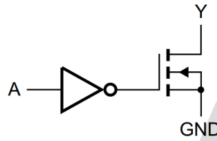
Figure 2. Logic diagram (one gate)
